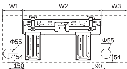
GWH18QDXD-K6DNC2I/I
