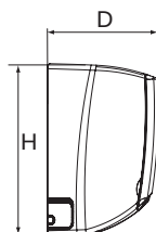
GWH09QCXB-K6DNC2F/I GWH12QCXB-K6DNC2F/I
