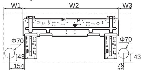
GWH24QEXF-K6DNC2I/I
