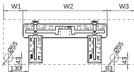
GWH24QEXF-K6DNC2I/I
